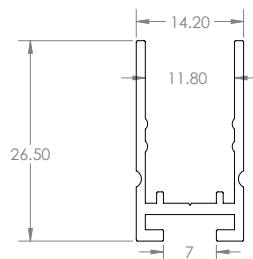
PZM-NFL-CHAN-4 Dimensions
